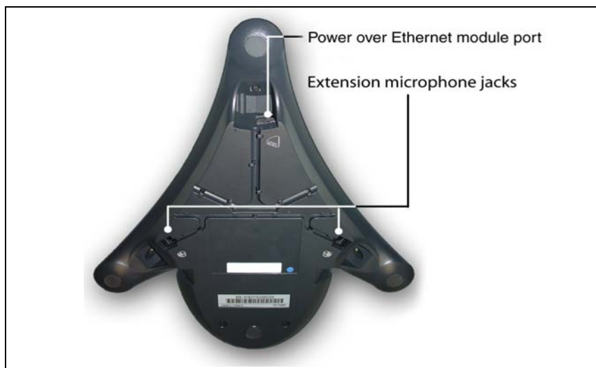
Figure 6: IP Audio Conference Phone 2033 connections
